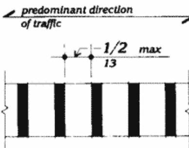
Fig. 8 (g) Gratings
