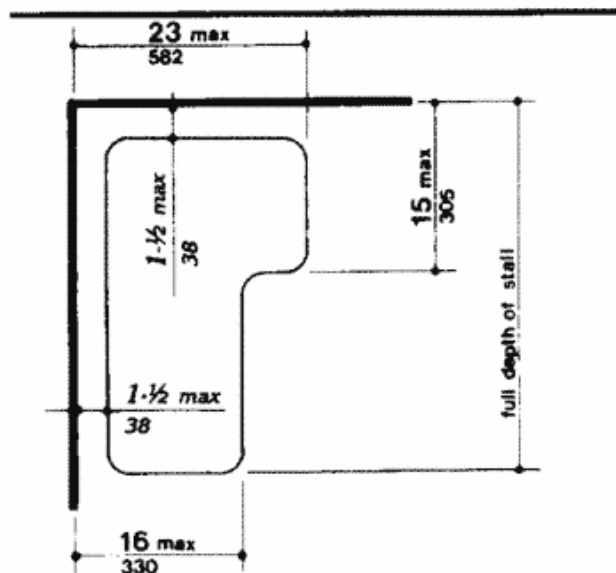
Fig. 36 Shower Seat Design
