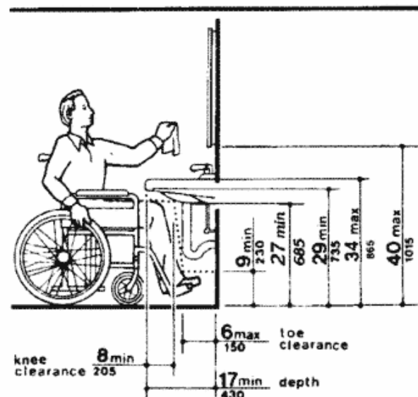
Fig. 31 Lavatory Clearances
