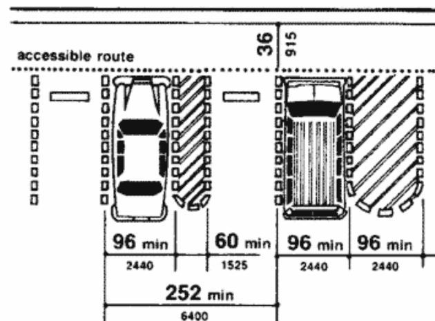
(a) Van Accessible Space at End Row
