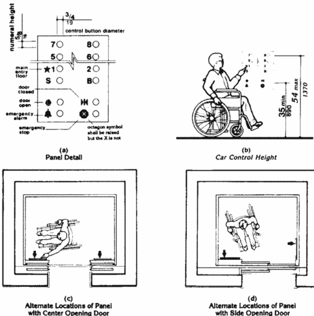
Fig. 23 Car Controls
