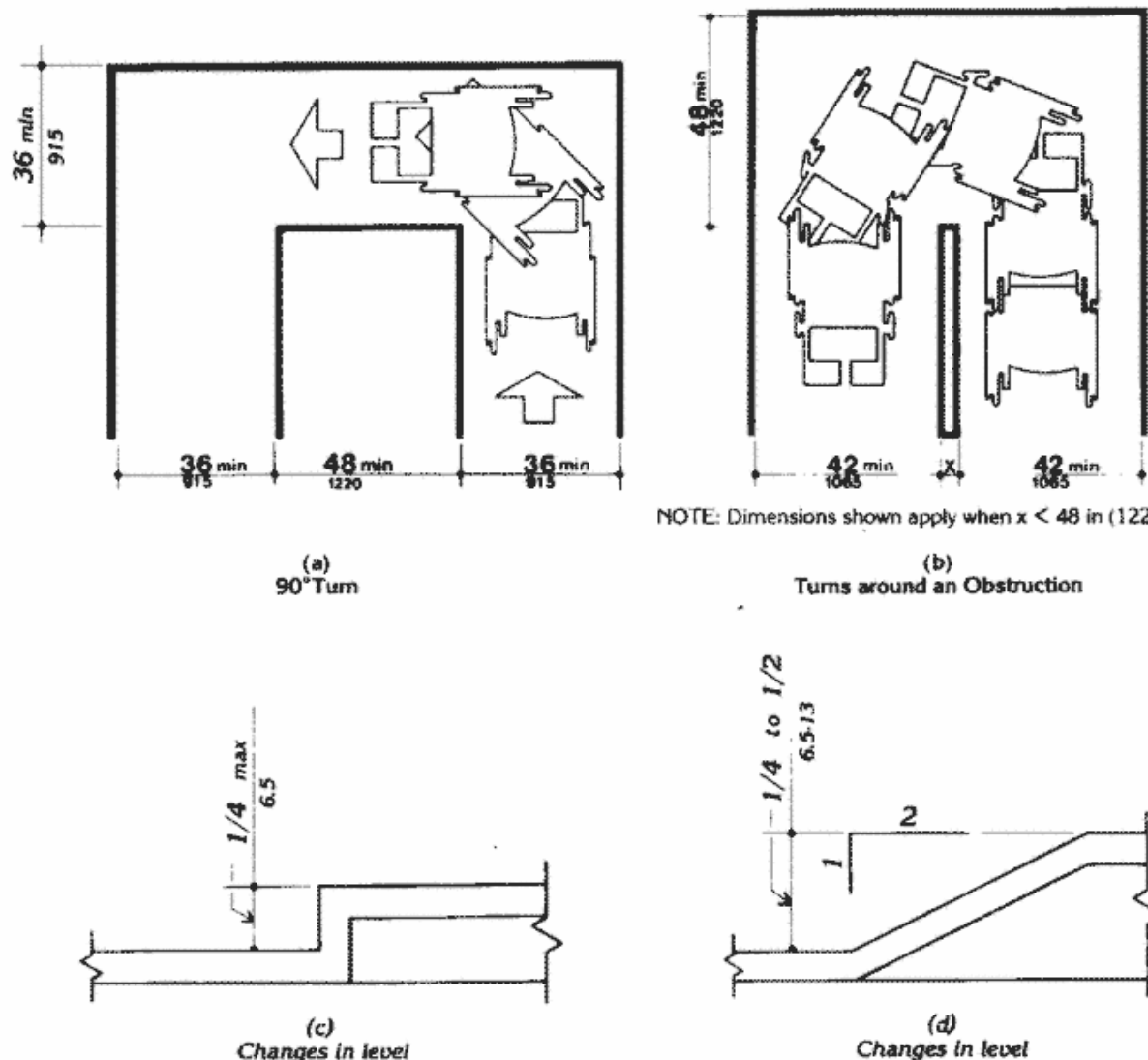
Fig. 7 Accessible Route
