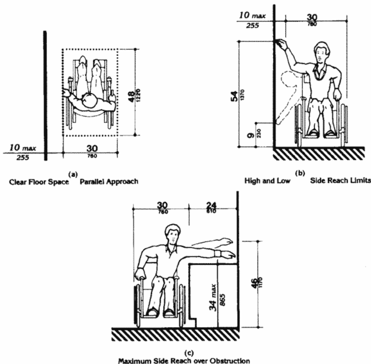
Fig. 6 Side Reach
