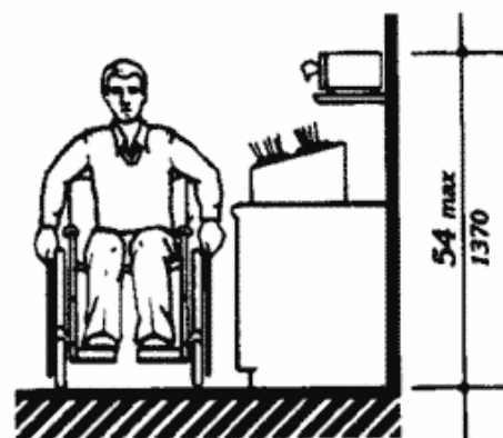
Fig. 54 Tableware Areas
