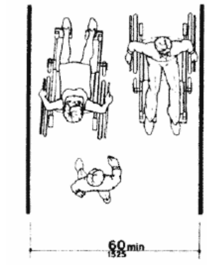
Fig. 2 Minimum Clear Width for Two Wheelchairs
