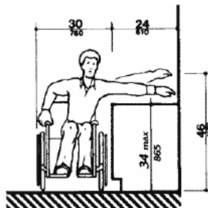
(c) Maximum Side Reach over construction
