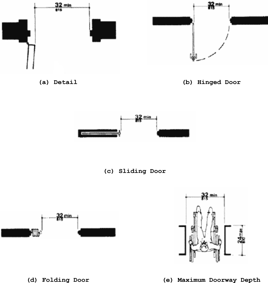
Fig. 24 Clear Doorway Width and Depth ("1991 Standards for Accessible Design", 28 CFR 36 Appendix D)
