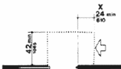
(f) Latch Side Approach - Sliding Doors and Folding Doors Fig. 25 Maneuvering Clearances at Doors
