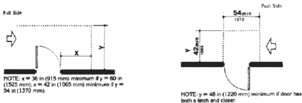
(b) Hinge Side Approaches - Swinging Doors
