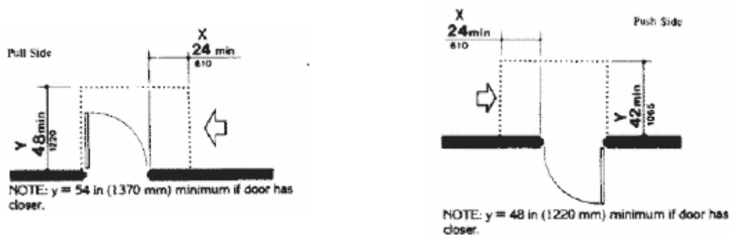
(c) Latch Side Approaches - Swinging Doors
