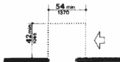
(e) Slide Approach - Sliding Doors and Folding Doors
