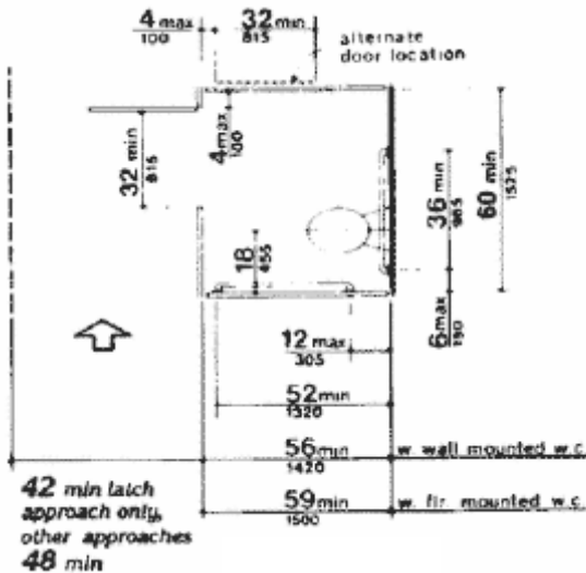
(a) Standard Stall
