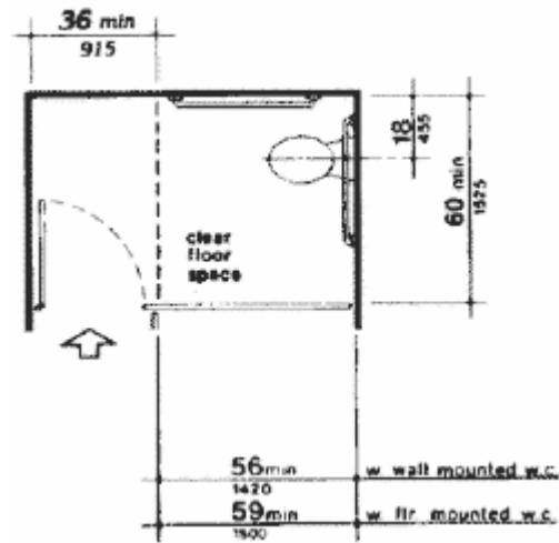
(a-1) Standard Stall (end of row)
