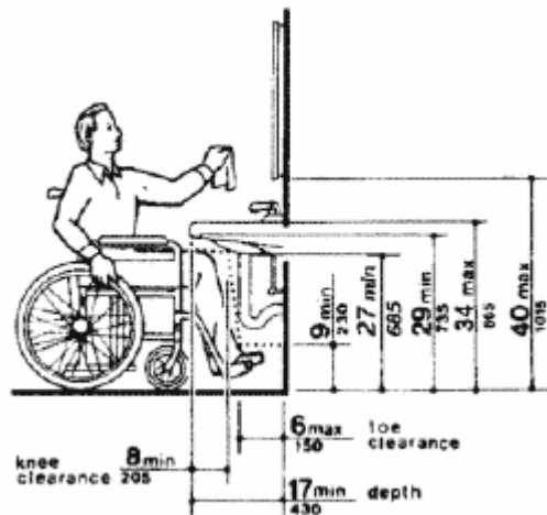
Fig. 31 Lavatory Clearances
