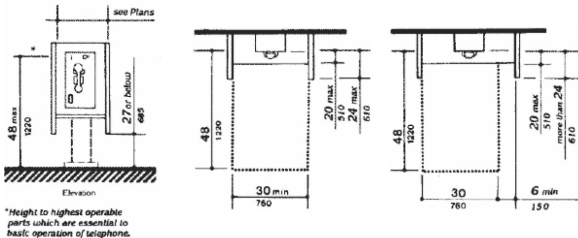
Fig. 44 Mounting Heights and Clearances for Telephones
