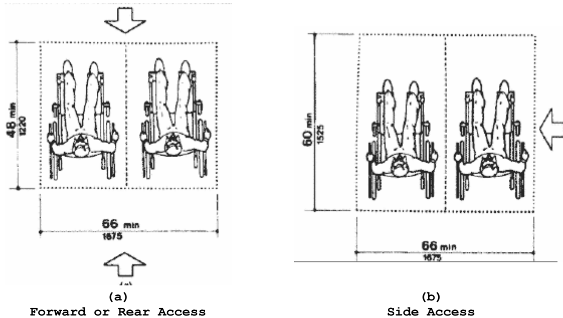
Fig. 46 Space Requirement for Wheelchair
