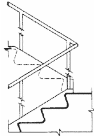
(b) Elevation of Center Handrail
