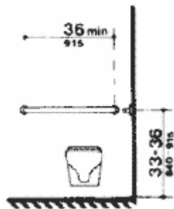
(c) Rear Wall of Standard Stall
