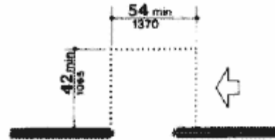
(e) Slide Approach - Sliding Doors and Folding Doors
