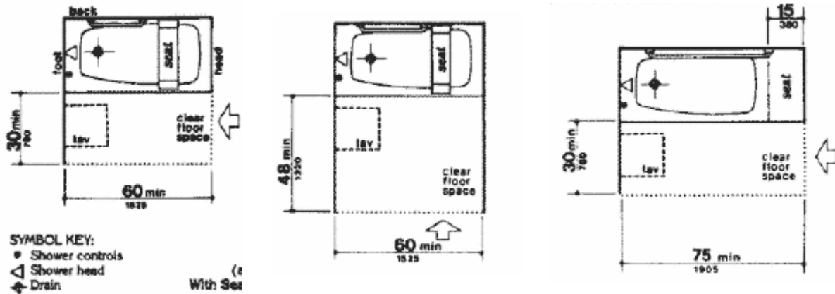
(a) (b) With Seat in Tub With Seat at Head of Tub Fig. 33 Clear Floor Space at Bathtubs
