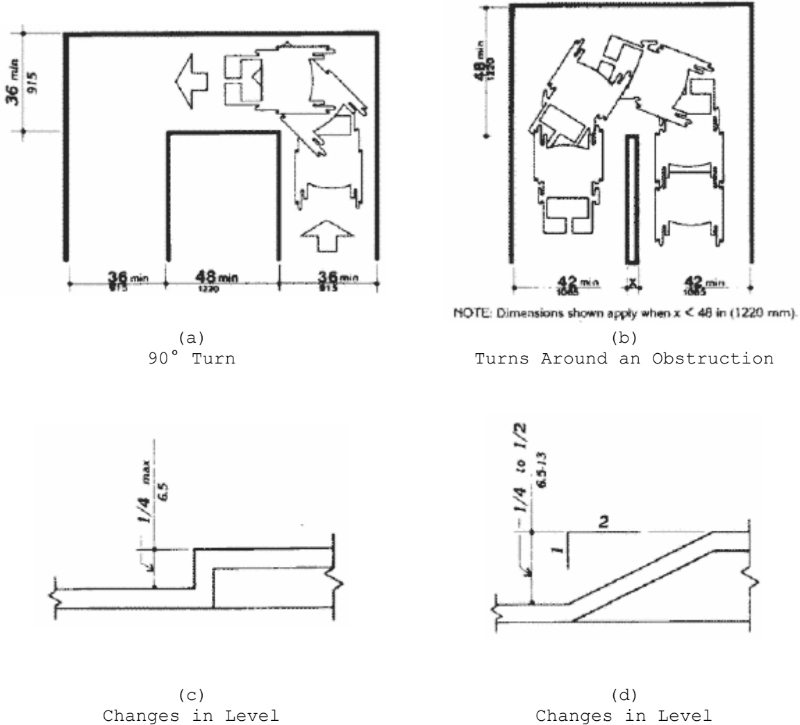
Fig. 7 Accessible Route
