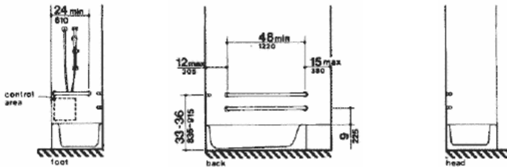
(b) With Seat at Head of Tub
