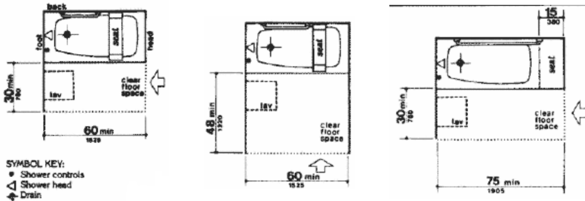
(a) Clear Floor Space at Bathtubs
