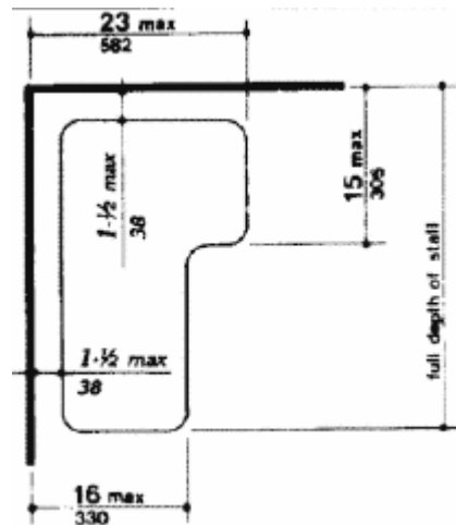
Fig. 36 Shower Seat Design
